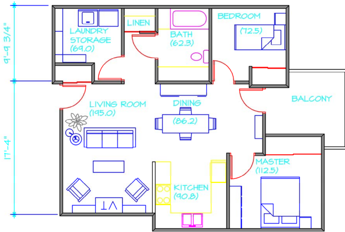
SECOND FLOOR UNIT GROSS UNIT AREA = 897.4 SF
