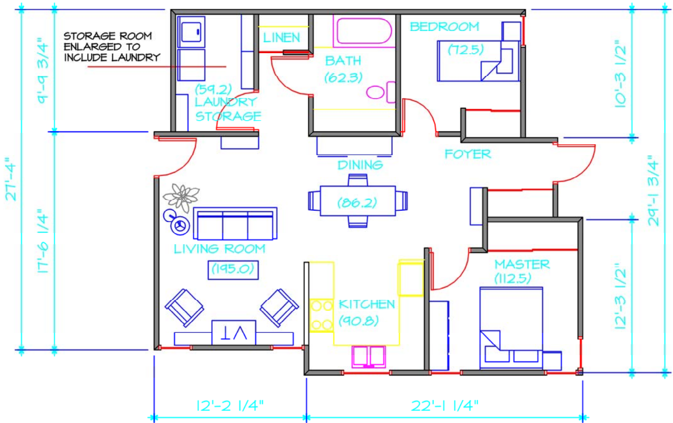
MAIN FLOOR UNIT GROSS UNIT AREA = 908.8 SF
