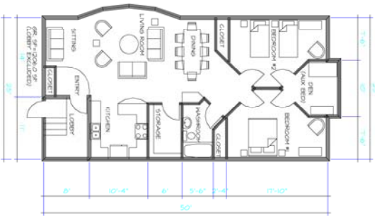
4 MIDDLE LEVEL FLOOR PLAN - 1/8
