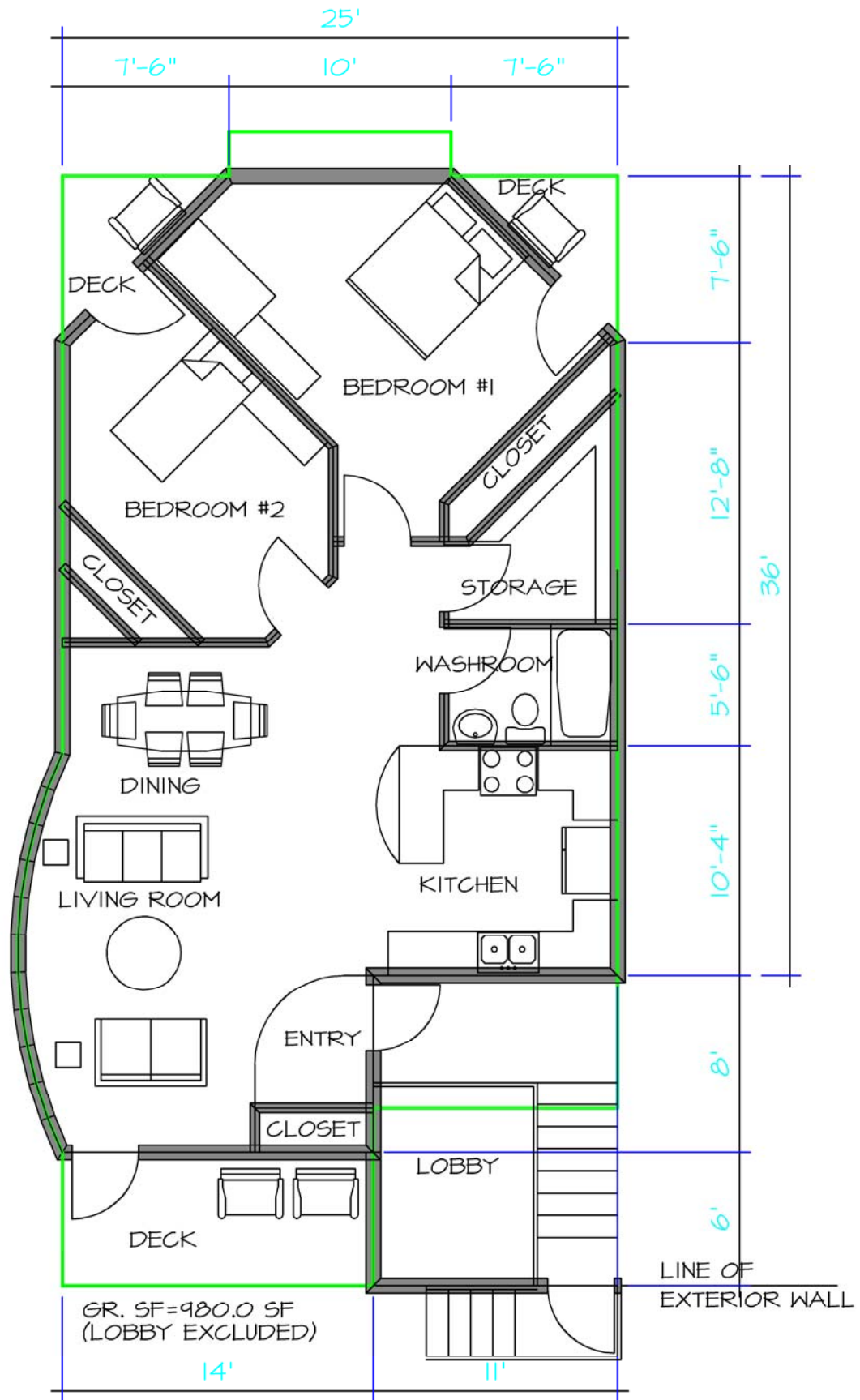
MIDDLE LEVEL FLOOR PLAN - 1/8
